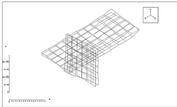
(b) Second mode at 90.0 Hz
