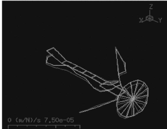
(b) Bouncing of a rear suspension at 35.1 Hz
