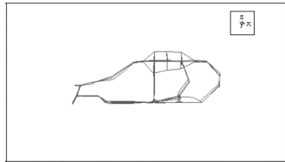
(b) Roof (0,1) mode shape at 48.7 Hz
