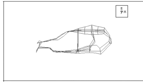
(a) Torsion and bending mode shape at 38.8 Hz
