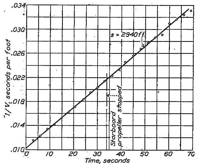
FIGURE 15.—ZMC-2 deceleration test. Run No. 4
