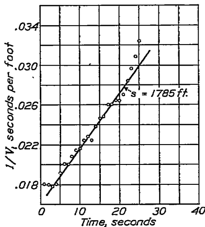
FIGURE 22.—TE-2 deceleration test. Run No. 4
