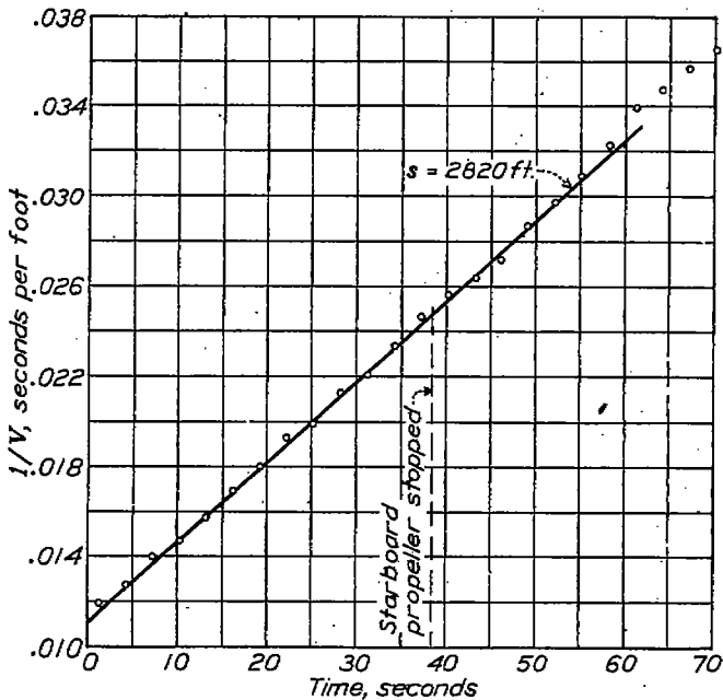
FIGURE 13.—ZMC-2 deceleration test. Run No. 2
