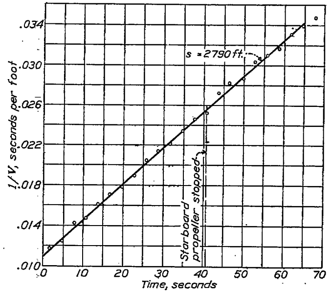
FIGURE 14.—ZMC-2 deceleration test. Run No. 3
