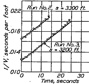
FIGURE 18.—TC-6 deceleration test. Run Nos. 2 and 3
