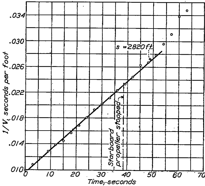
FIGURE 12.—ZMC-2 deceleration test. Run No. 1
