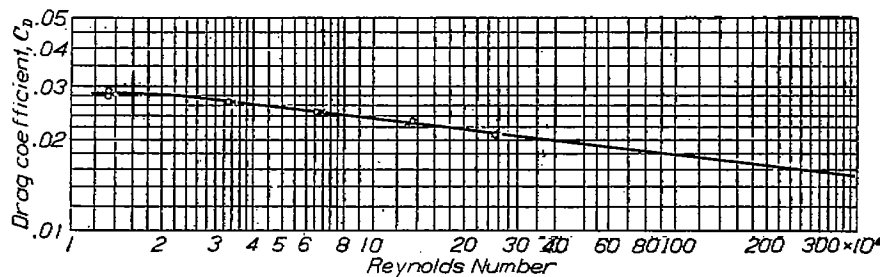
FIGURE 25.—Drag coefficient versus Reynolds Number for a bare-bull airship model. (Length-diameter ratio=5.0)
