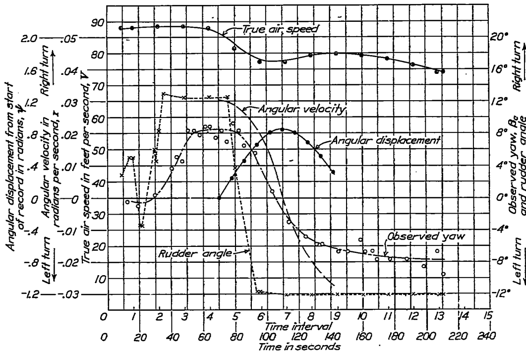
FIGURE 7.—Run No. 17D. Reversal—right to left. Altitude referred to standard atmosphere=8,030 feet
