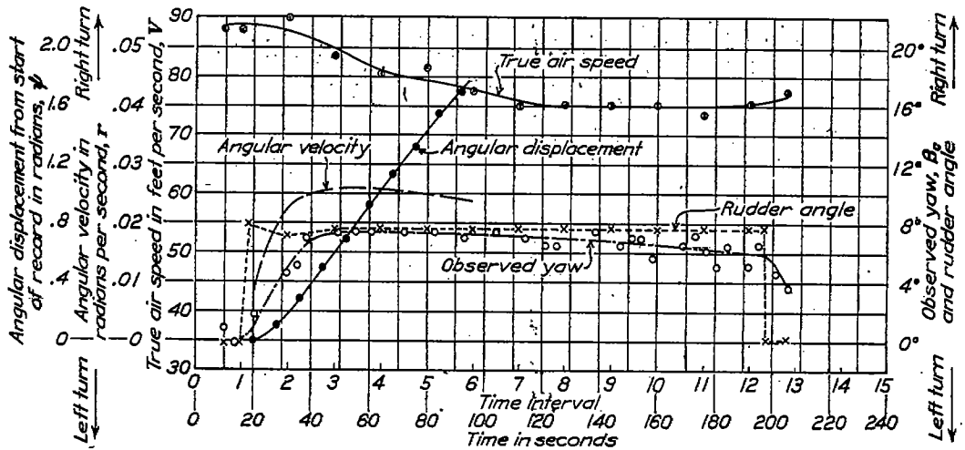
FIGURE 4.—Run No. 50. Right turn. Altitude referred to standard atmosphere=3,080 feet
