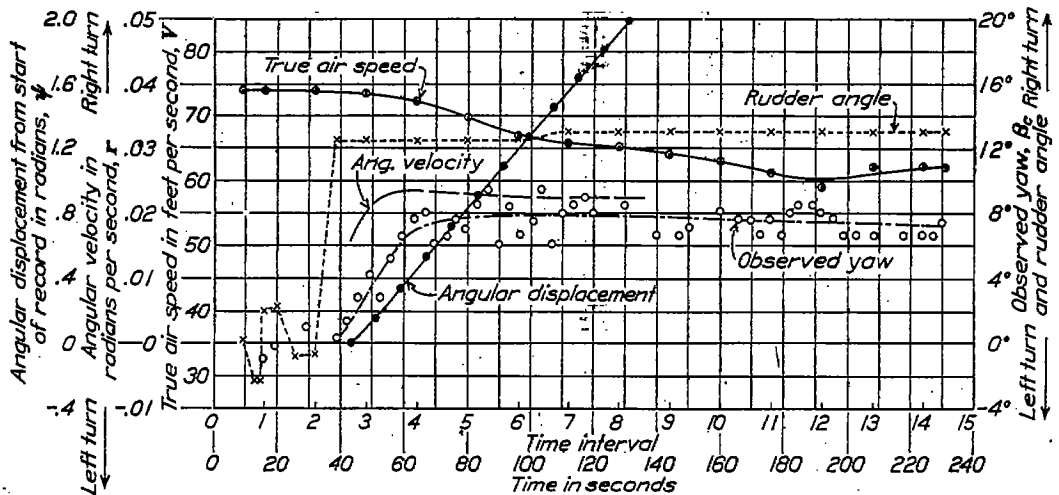
FIGURE 5.—Run No. 18D. Right turn. Altitude referred to standard atmosphere=3,030 feet
