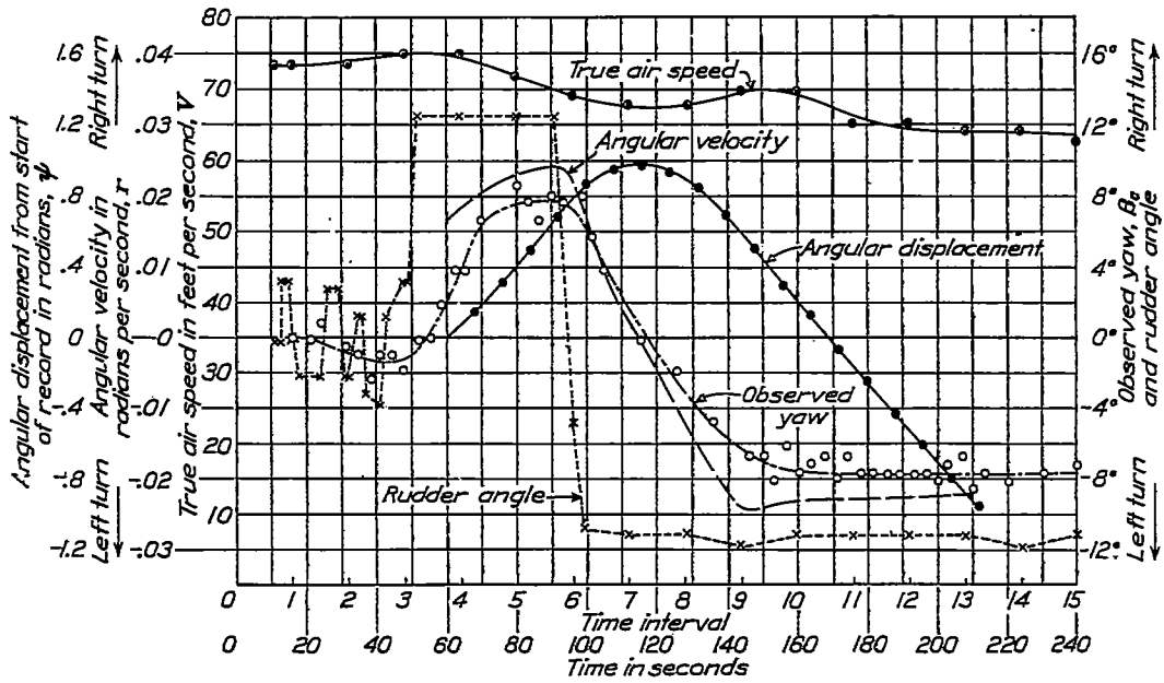
FIGURE 6.—Run No. 14D. Reversal—right to left. Altitude referred to standard atmosphere=8,030 feet
