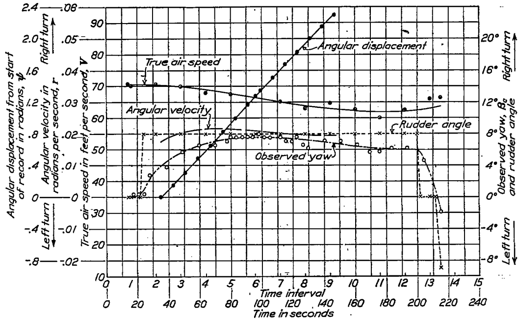
FIGURE 3.—Run No. 40. Right turn. Altitude referred to standard atmosphere=3,080 feet
