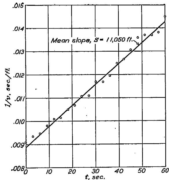
FIGURE 20.—Run No. 3. Deceleration without water recovery. Propellers idling. Speeds by N. A. C. A. recording instrument
