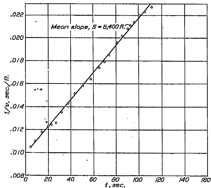
FIGURE 10.—Run No. 5. Deceleration with water recovery. Propellers stopped. Speed by electric meter
