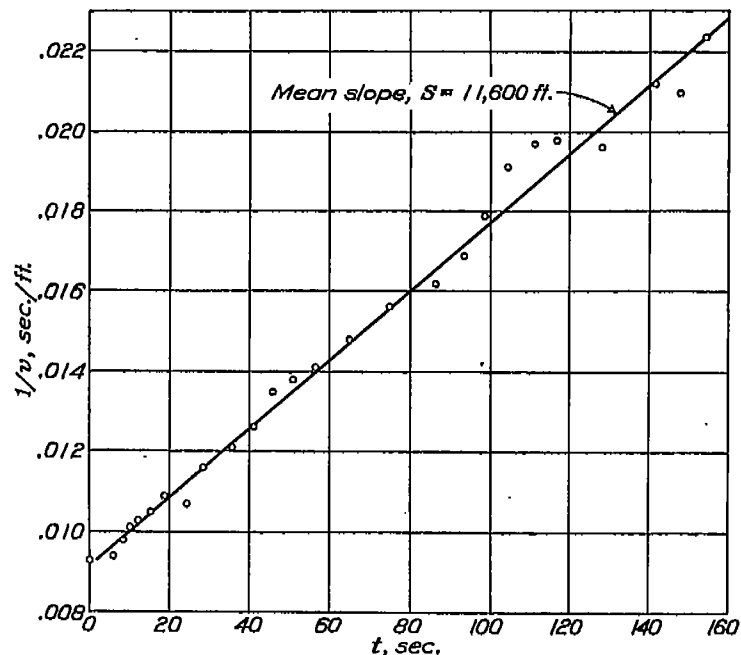
FIGURE 2.—Run No. 1. Deceleration without water recovery. Propellers stopped. Speeds by electric meter
