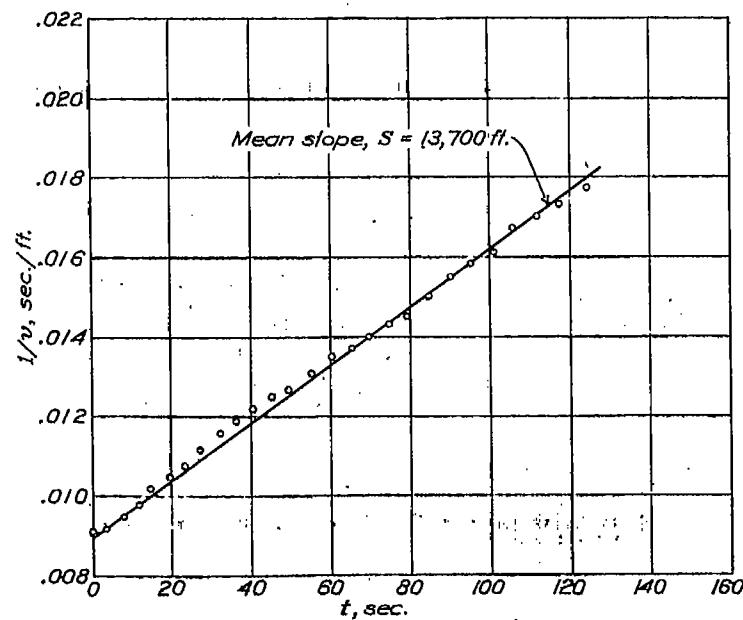
FIGURE 9.—Run No. 4. Deceleration without water recovery. Propellers idling. Speeds by Venturi meter
