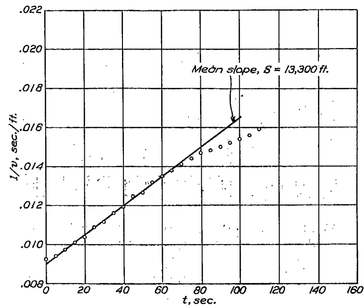
FIGURE 7.—Run No. 2. Deceleration without water recovery. Propellers stopped. Speeds by Venturi meter
