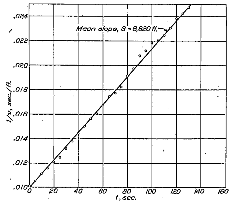
FIGURE 13.—Run No. 8. Deceleration with water recovery. Propellers idling. Speeds by electric meter
