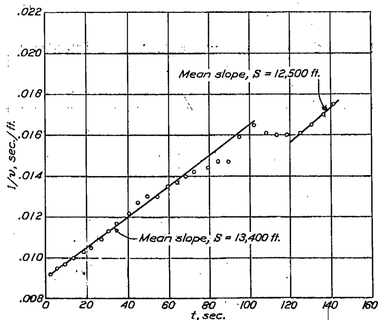
FIGURE 8.—Run No. 2. Deceleration without water recovery. Propellers idling. Speeds by Venturi meter
